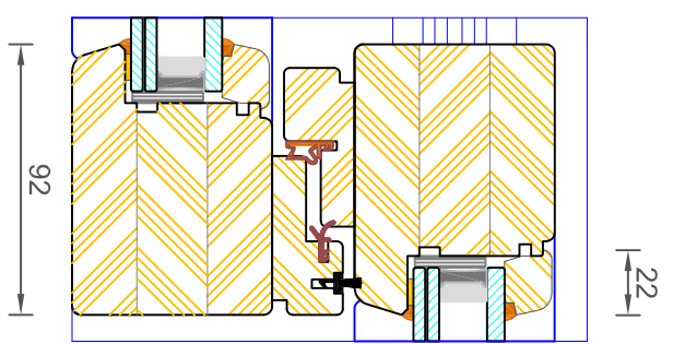
Section B-B
