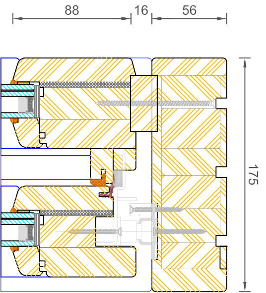
Section F-F
