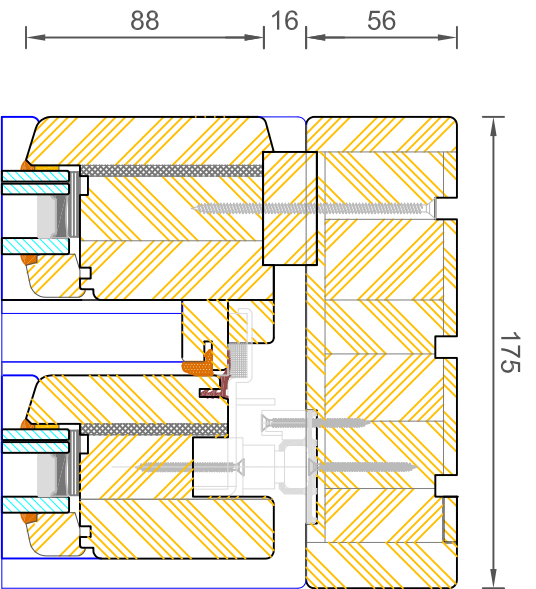
Section F-F
