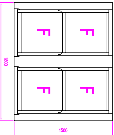
fixed sash - fixed sash / fixed sash - fixed sash
