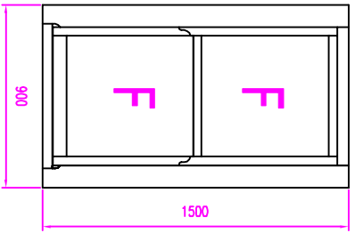
fixed sash / fixed sash
