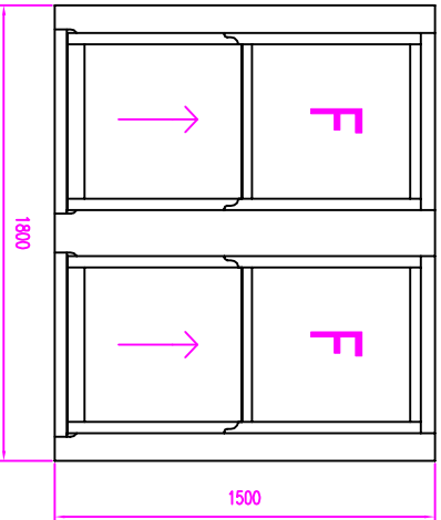
fixed sash - fixed sash / sash - sash
