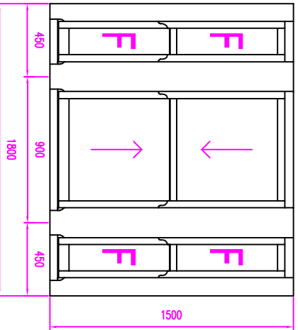
fixed sash - sash - fixed sash / fixed sash - sash - fixed sash
